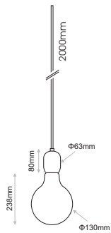
\Phi 130 \times 238 (h)
