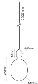
\Phi 170 \times 270 (h)
