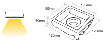
PCR.005 SEAMLESS SQUARE ADJUSTABLE
